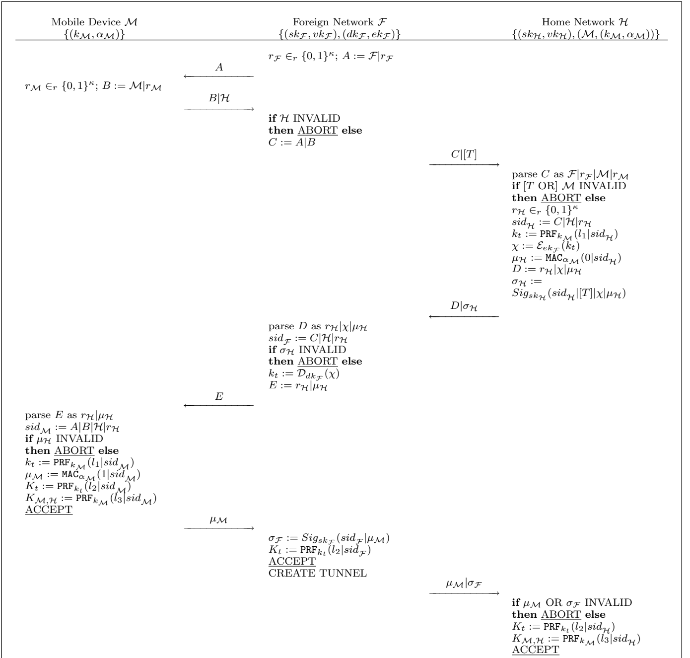
Figure 1: Illustration of the basic version of AWRT between the participating mobile device \mathcal{M} , foreign network \mathcal{F} , and home network \mathcal{H} . At the end of the protocol: \mathcal{M} and \mathcal{H} hold the end-to-end key K_{\mathcal{M}, \mathcal{H}} ; \mathcal{M} , \mathcal{F} , and \mathcal{H} hold the tunnel key K_t , so that the tunnel between \mathcal{M} and \mathcal{H} can be established by \mathcal{F} .
