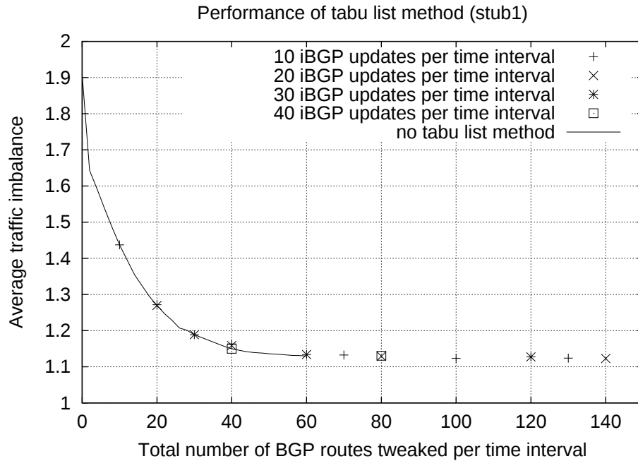
Figure 6.8: Performance of tabu list method with last value predictor.
