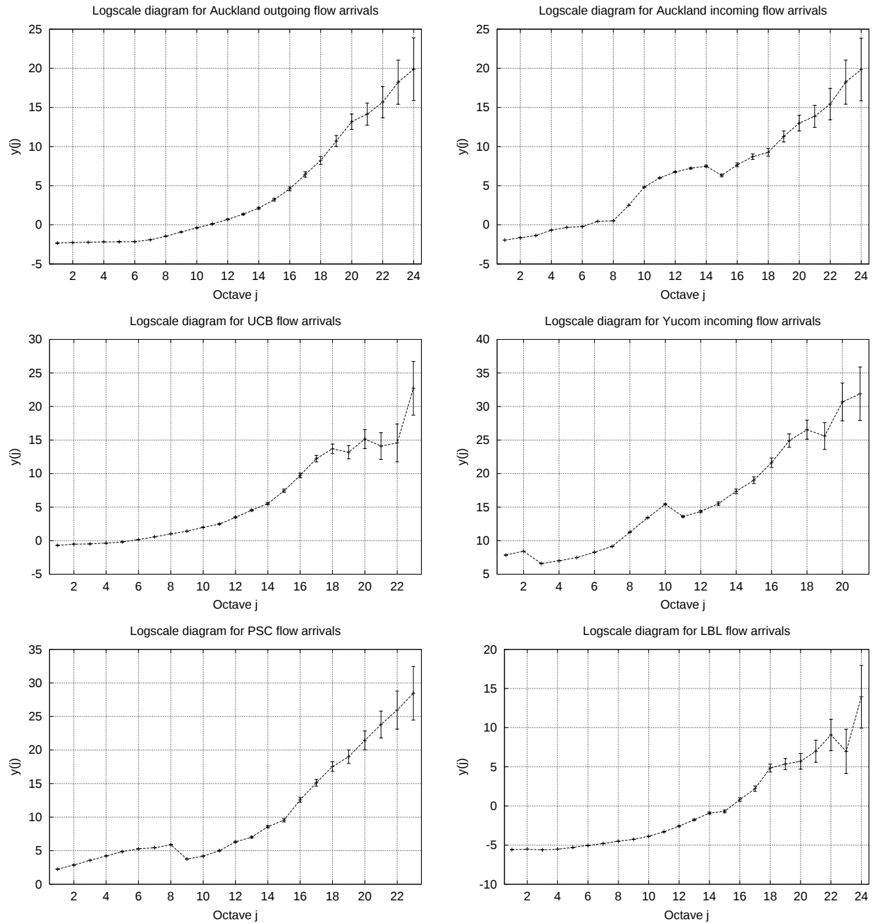
Figure 1.8: Logscale diagrams.
