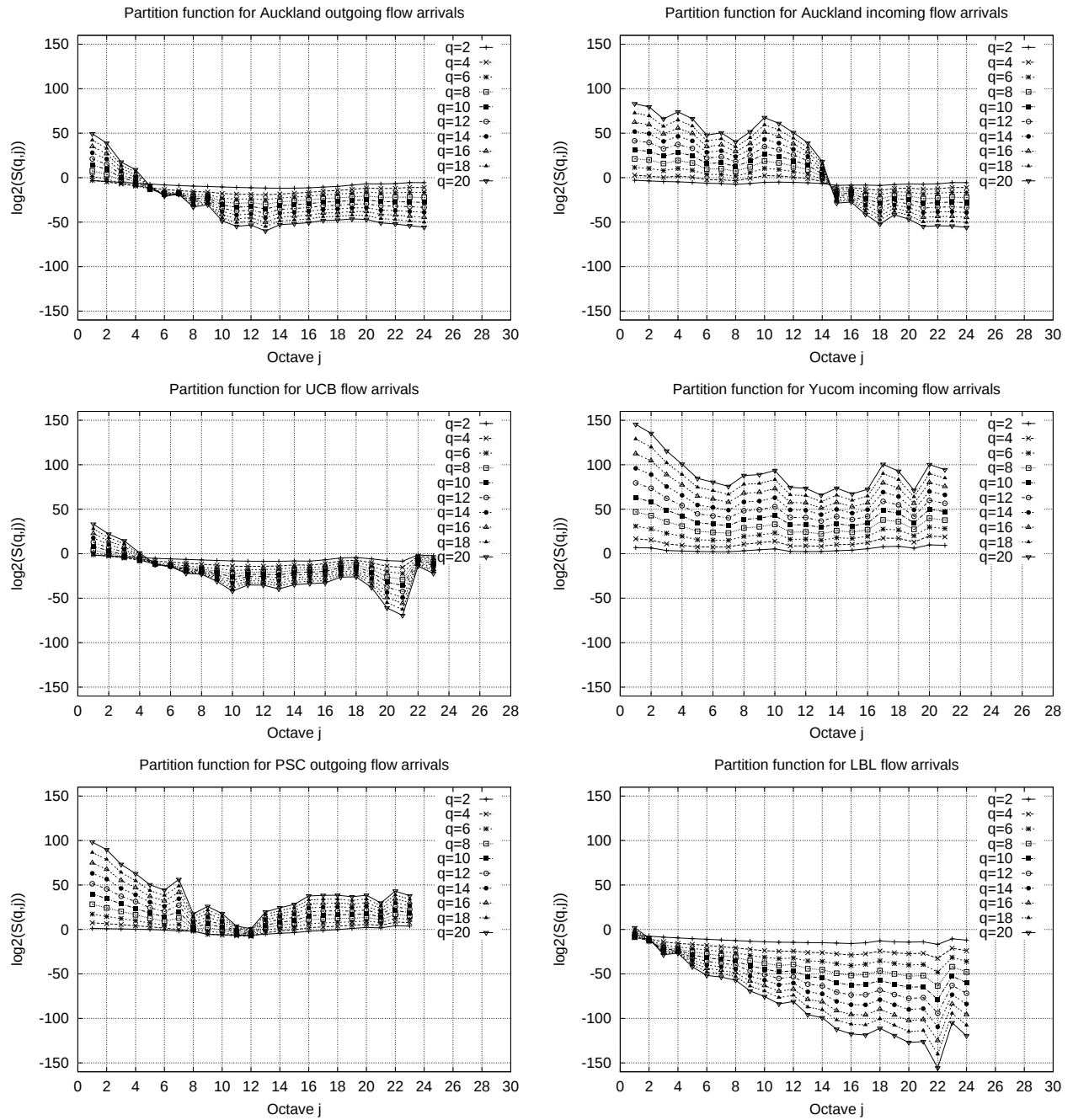
Figure 1.10: Partition functions.
