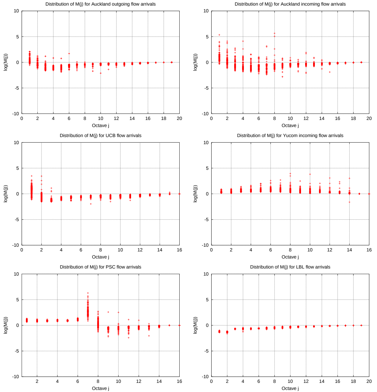
Figure 1.12: M(j) estimator.
