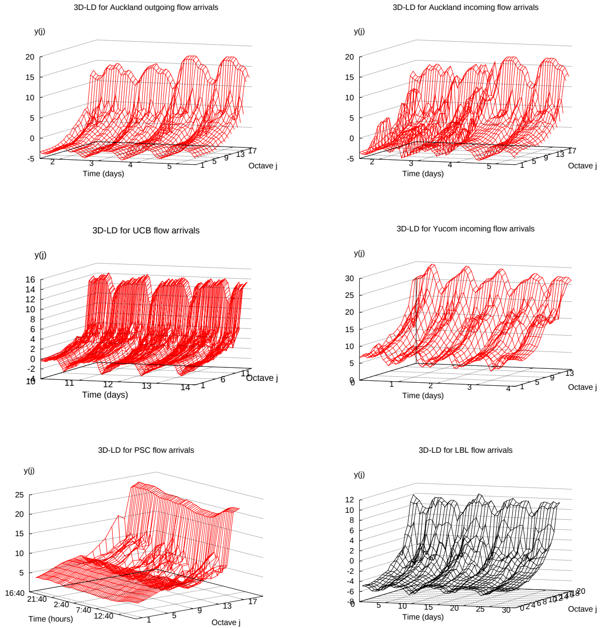
Figure 1.9: 3D-logscale diagrams.
