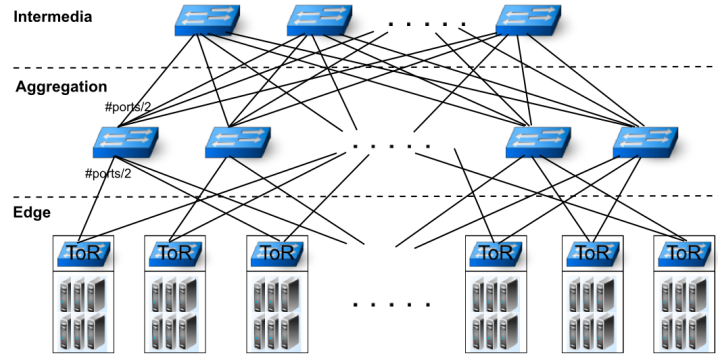
Figure 4.2: Cloud DC
