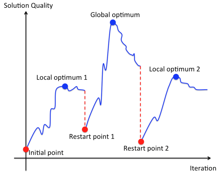
Figure 2.8: Local Search
