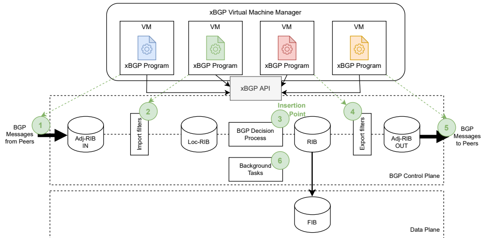
Figure 1: An xBGP compliant implementation exposes the abstract BGP data structures defined in RFC4271 through a generic API and uses libxbgp’s Virtual Machine Manager to attach the bytecode that implements extensions to specific insertion points (green circles). The four bytecodes in this example support a simple GeoLoc BGP attribute. For each xBGP program, we provide the set of helper functions used to retrieve data from the host implementation.
