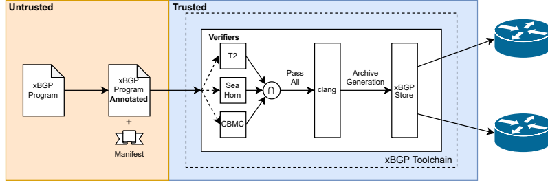
Figure 2: High-level view of the xBGP verification toolchain.
