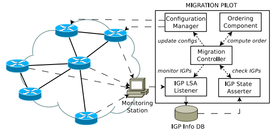
Figure 9: System architecture.
