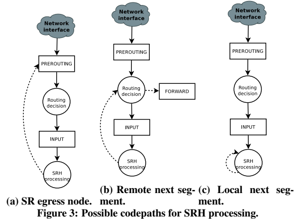
Figure 3: Possible codepaths for SRH processing.
