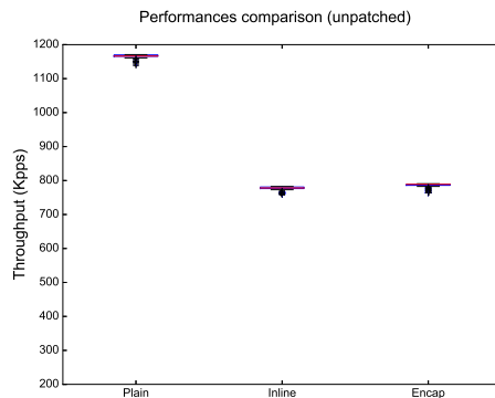
Figure 5: Initial performances for encapsulation and insertion.
